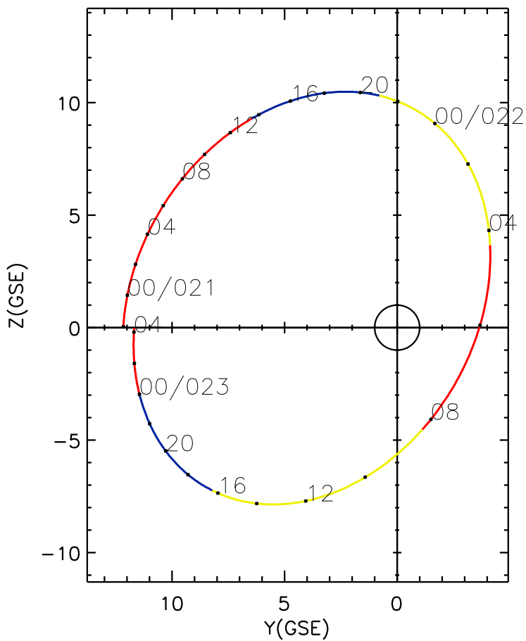
CLUSTER 2 orbit 2020 020 (01/20) 21:56 UT to 2020 023 (01/23) 04:16 UT
