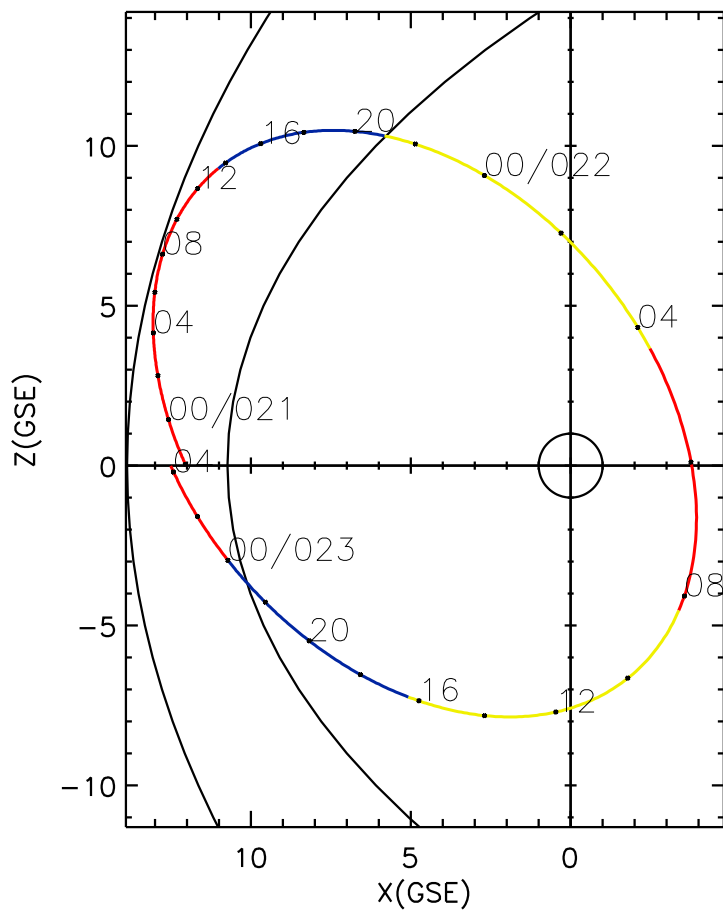
CLUSTER 2 orbit 2020 020 (01/20) 21:56 UT to 2020 023 (01/23) 04:16 UT
