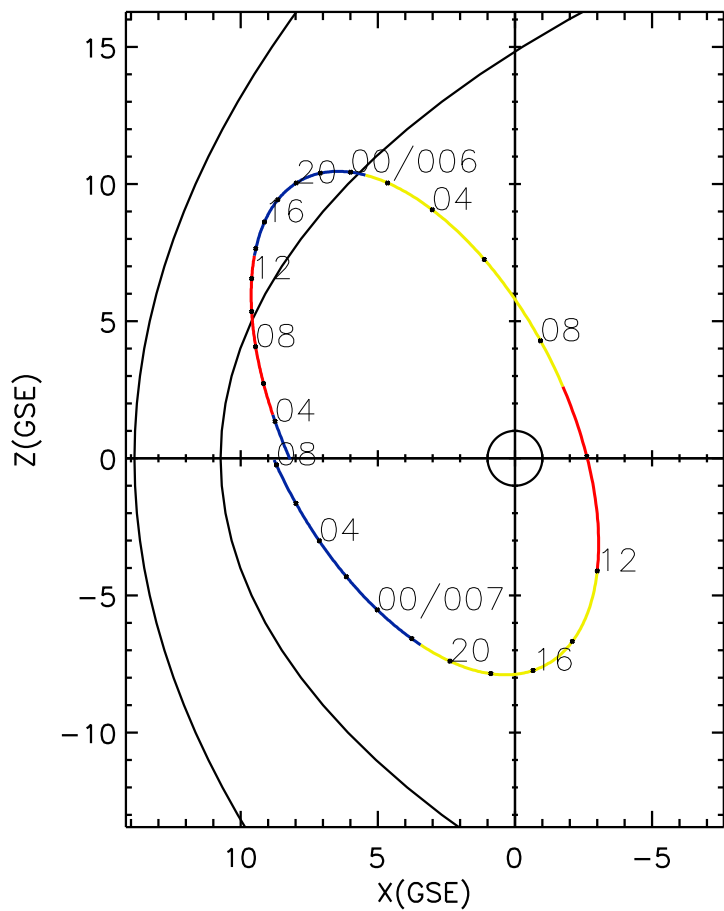
CLUSTER 2 orbit 2020 005 (01/05) 02:01 UT to 2020 007 (01/07) 08:16 UT
