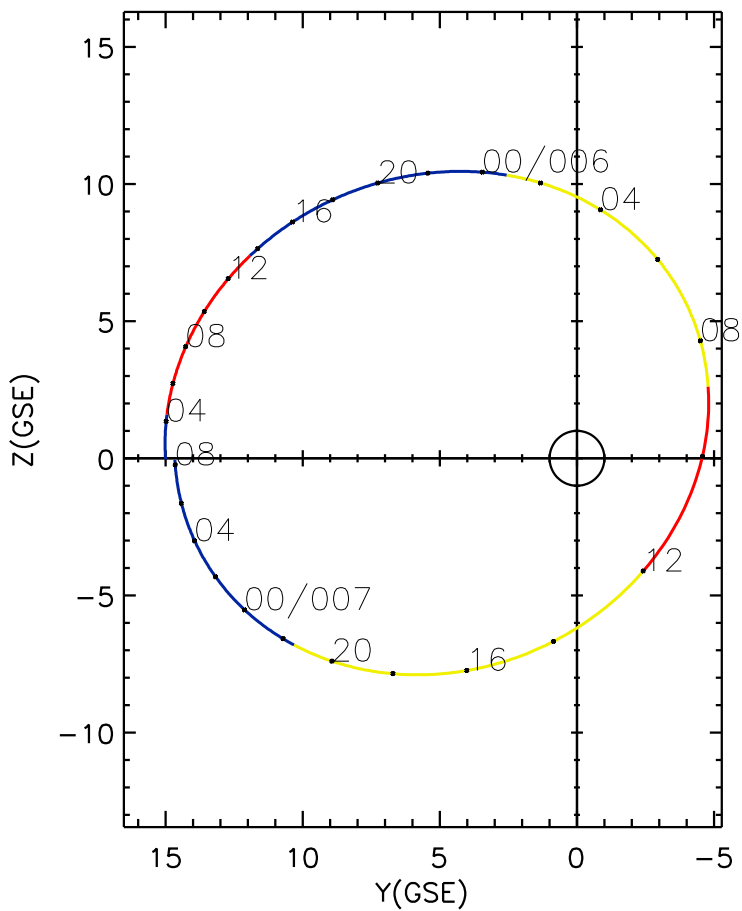
CLUSTER 2 orbit 2020 005 (01/05) 02:01 UT to 2020 007 (01/07) 08:16 UT
