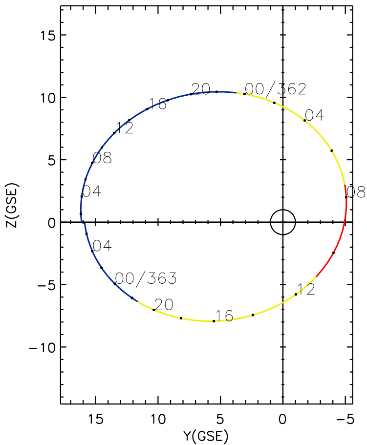
CLUSTER 2 orbit 2019 361 (12/27) 01:01 UT to 2019 363 (12/29) 07:16 UT
