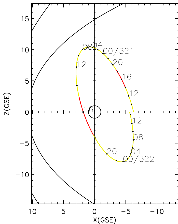
CLUSTER 2 orbit 2019 320 (11/16) 08:16 UT to 2019 322 (11/18) 14:31 UT
