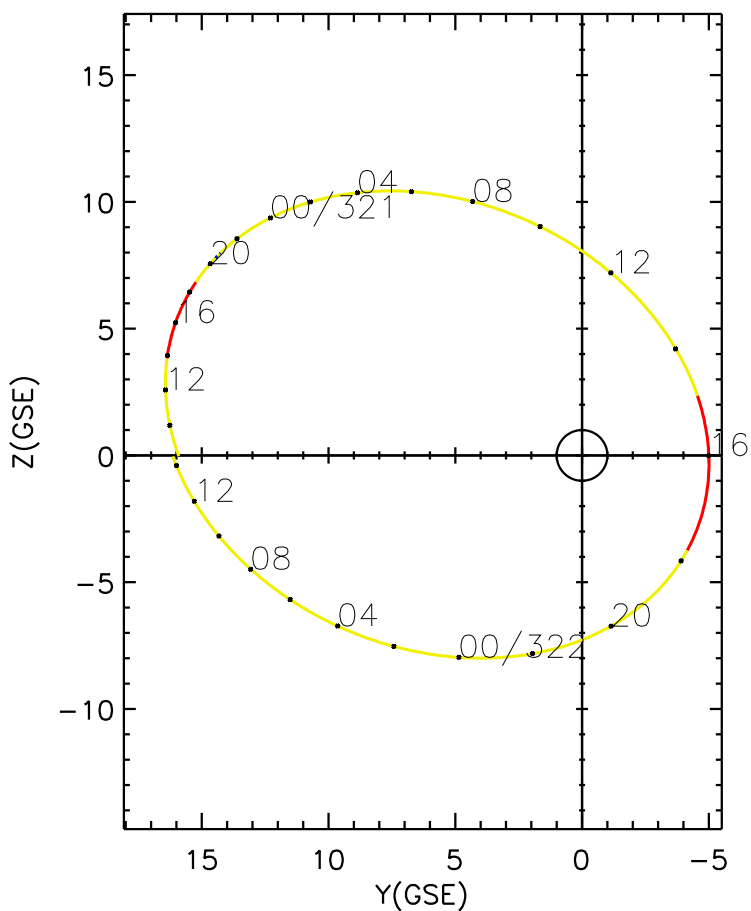
CLUSTER 2 orbit 2019 320 (11/16) 08:16 UT to 2019 322 (11/18) 14:31 UT
