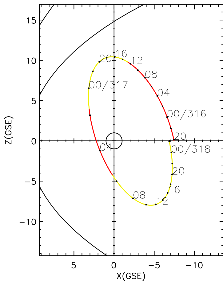
CLUSTER 2 orbit 2019 315 (11/11) 19:41 UT to 2019 318 (11/14) 02:01 UT
