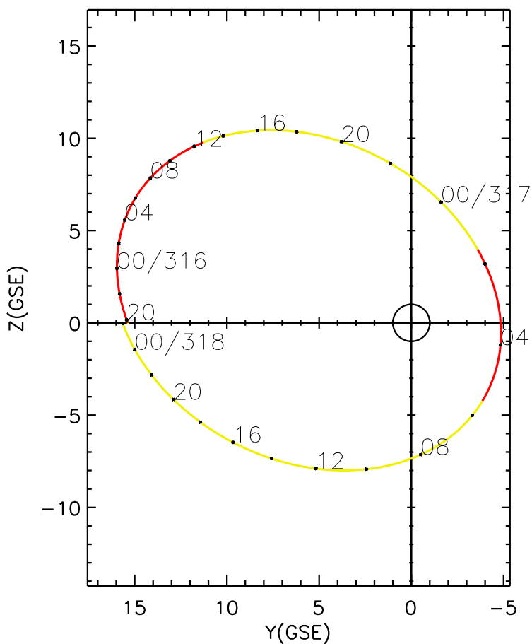
CLUSTER 2 orbit 2019 315 (11/11) 19:41 UT to 2019 318 (11/14) 02:01 UT
