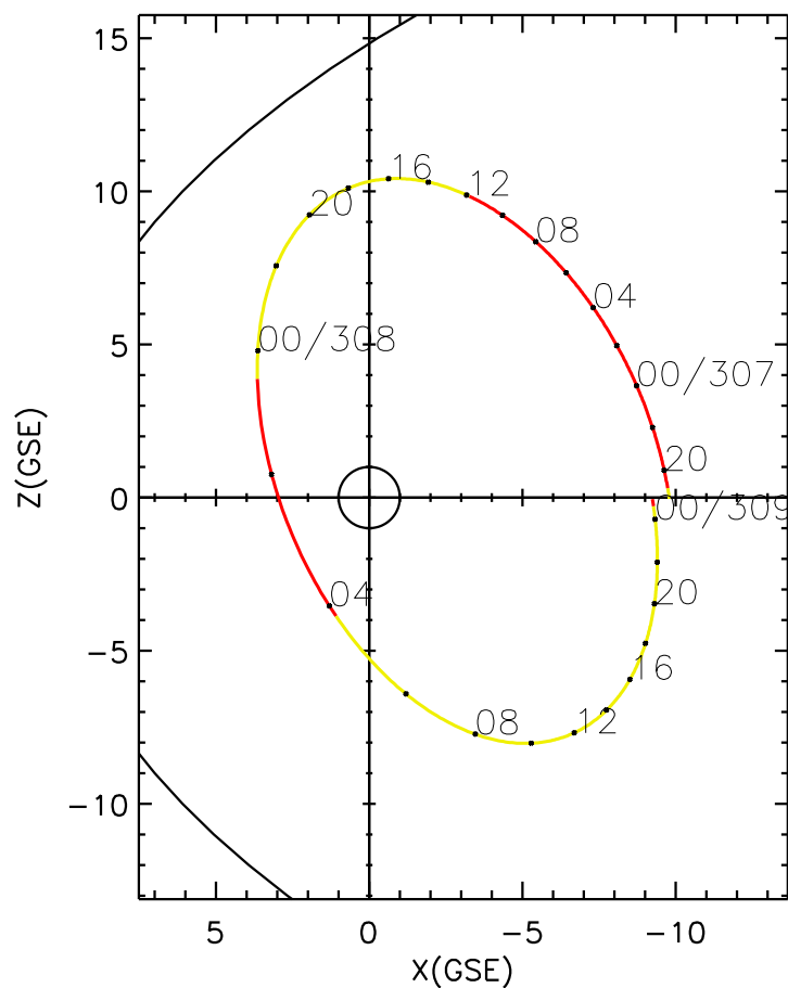
CLUSTER 2 orbit 2019 306 (11/02) 18:41 UT to 2019 309 (11/05) 00:56 UT
