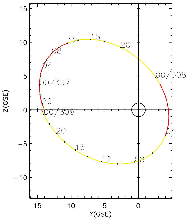
CLUSTER 2 orbit 2019 306 (11/02) 18:41 UT to 2019 309 (11/05) 00:56 UT
