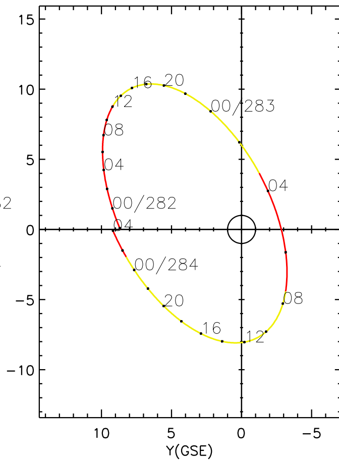
CLUSTER 2 orbit 2019 281 (10/08) 21:51 UT to 2019 284 (10/11) 04:06 UT
