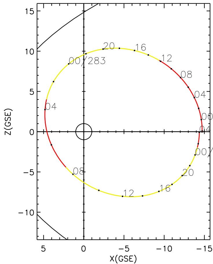
CLUSTER 2 orbit 2019 281 (10/08) 21:51 UT to 2019 284 (10/11) 04:06 UT
