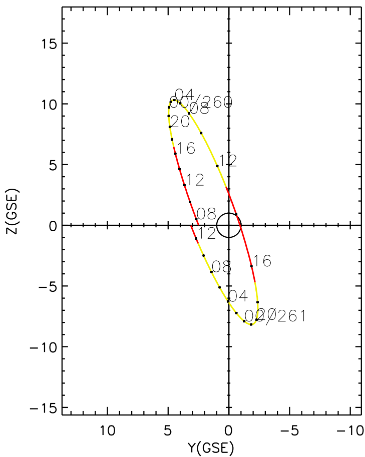
CLUSTER 2 orbit 2019 259 (09/16) 07:16 UT to 2019 261 (09/18) 13:31 UT
