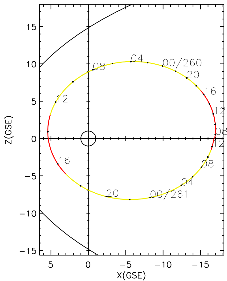
CLUSTER 2 orbit 2019 259 (09/16) 07:16 UT to 2019 261 (09/18) 13:31 UT
