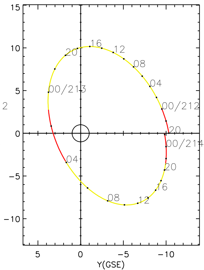
CLUSTER 2 orbit 2019 211 (07/30) 19:56 UT to 2019 214 (08/02) 02:11 UT
