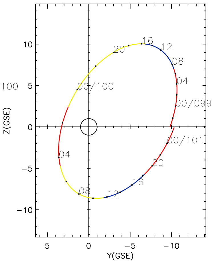
CLUSTER 2 orbit 2019 098 (04/08) 20:31 UT to 2019 101 (04/11) 02:41 UT
