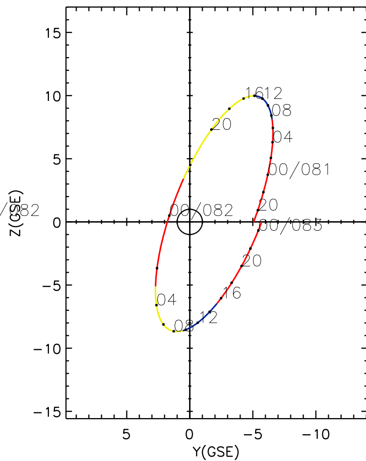
CLUSTER 2 orbit 2019 080 (03/21) 18:41 UT to 2019 083 (03/24) 00:56 UT
