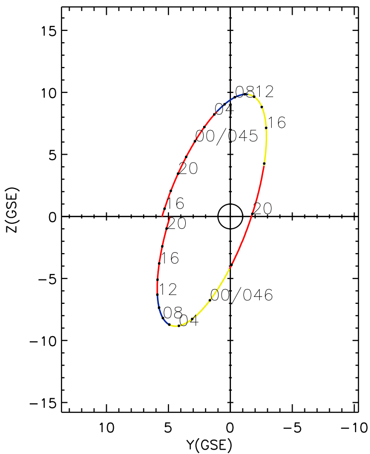
CLUSTER 2 orbit 2019 044 (02/13) 15:06 UT to 2019 046 (02/15) 21:21 UT
