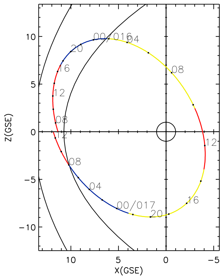
CLUSTER 2 orbit 2019 015 (01/15) 06:41 UT to 2019 017 (01/17) 12:51 UT
