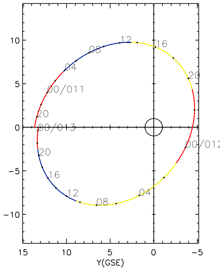
CLUSTER 2 orbit 2019 010 (01/10) 18:16 UT to 2019 013 (01/13) 00:31 UT
