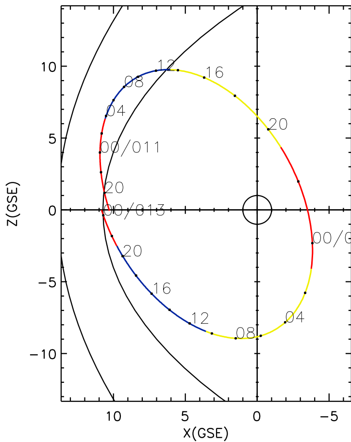
CLUSTER 2 orbit 2019 010 (01/10) 18:16 UT to 2019 013 (01/13) 00:31 UT
