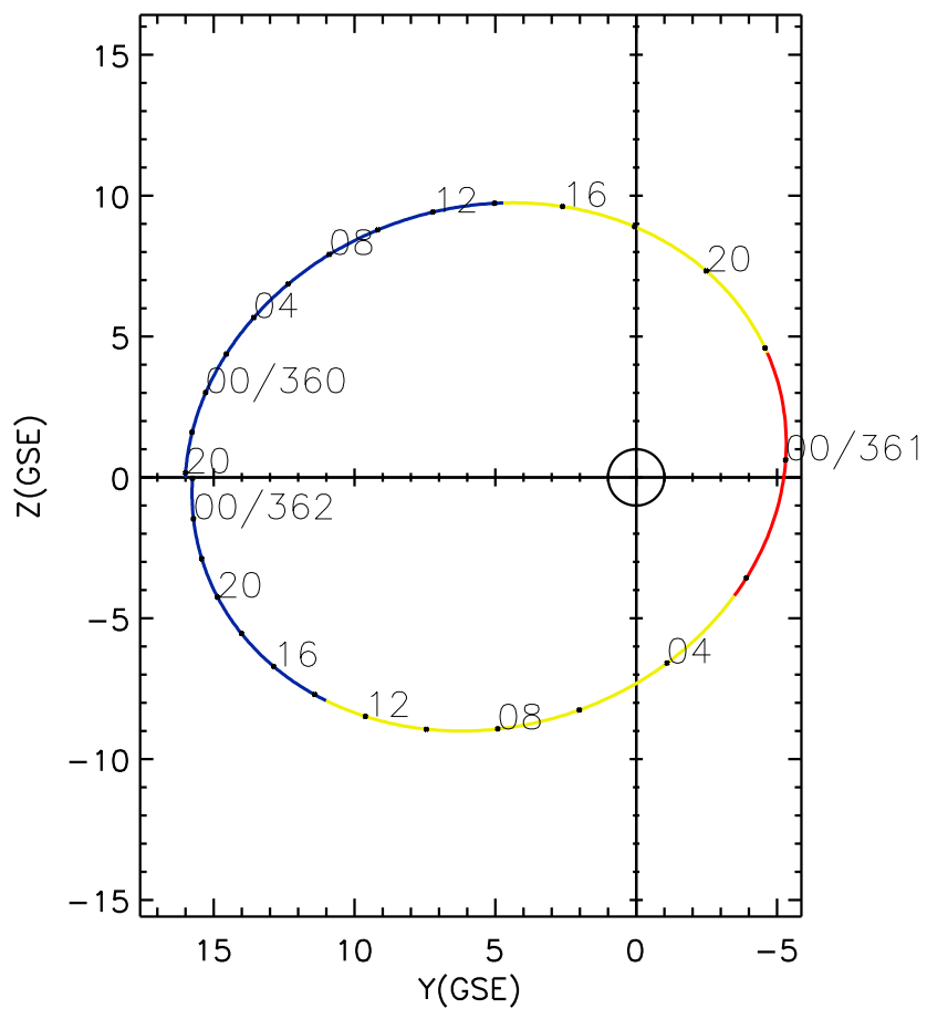
CLUSTER 2 orbit 2018 359 (12/25) 19:46 UT to 2018 362 (12/28) 02:01 UT
