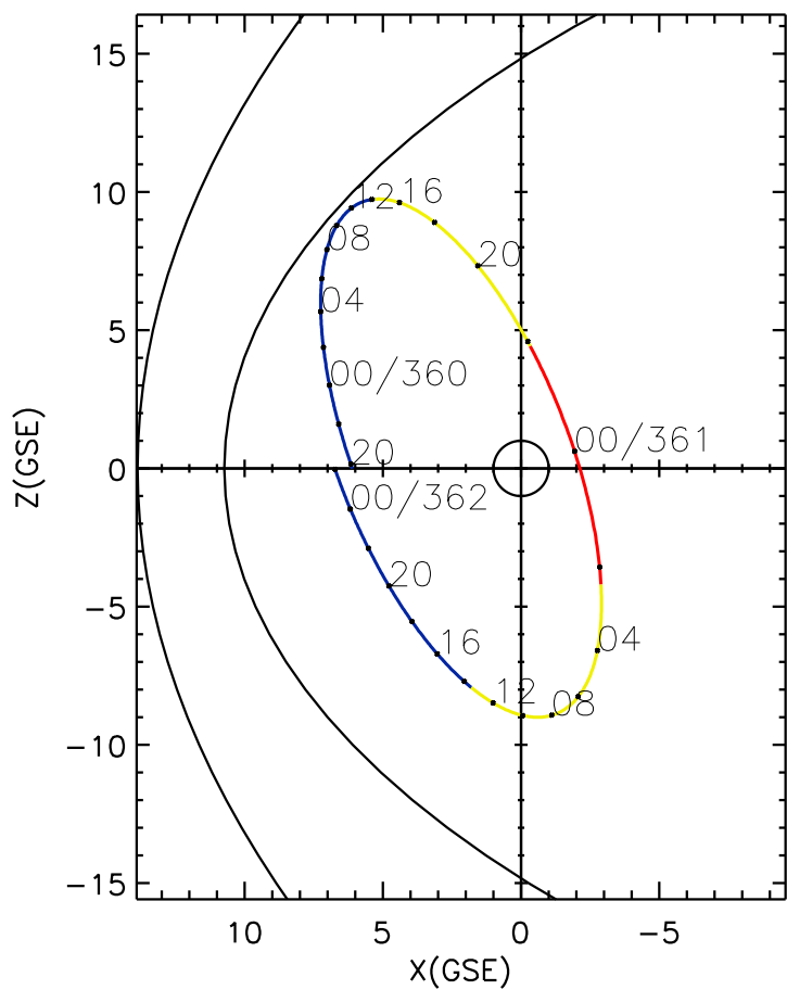
CLUSTER 2 orbit 2018 359 (12/25) 19:46 UT to 2018 362 (12/28) 02:01 UT
