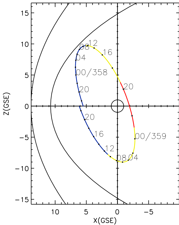
CLUSTER 2 orbit 2018 357 (12/23) 16:46 UT to 2018 359 (12/25) 23:01 UT
