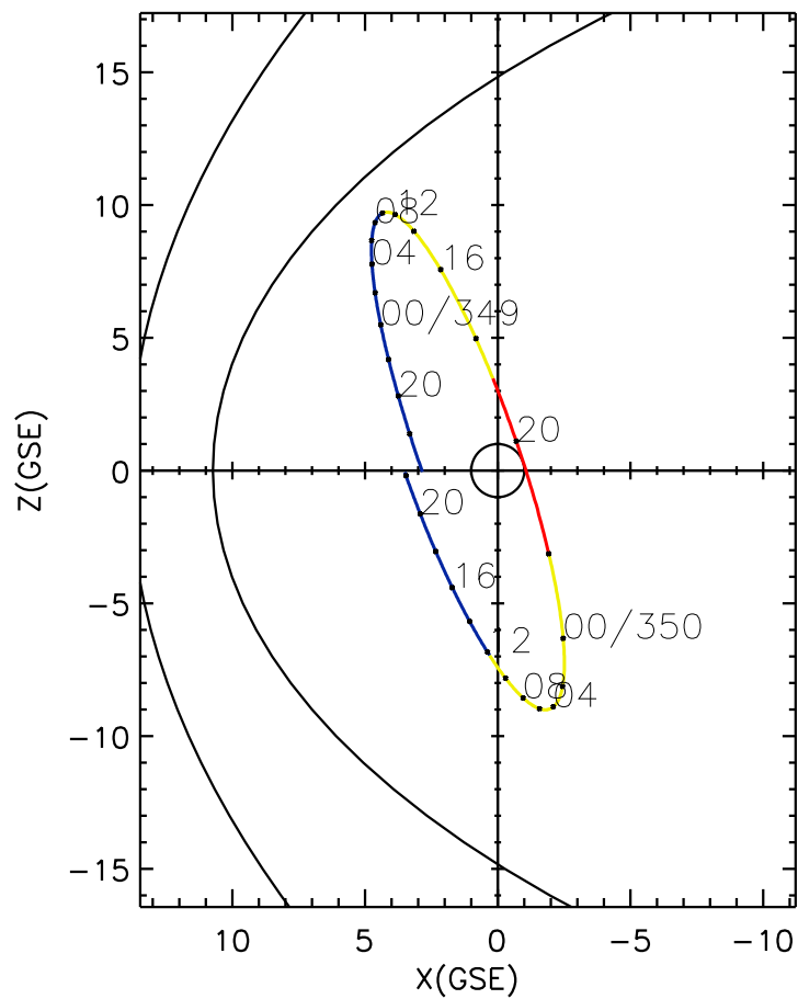
CLUSTER 2 orbit 2018 348 (12/14) 16:01 UT to 2018 350 (12/16) 22:11 UT
