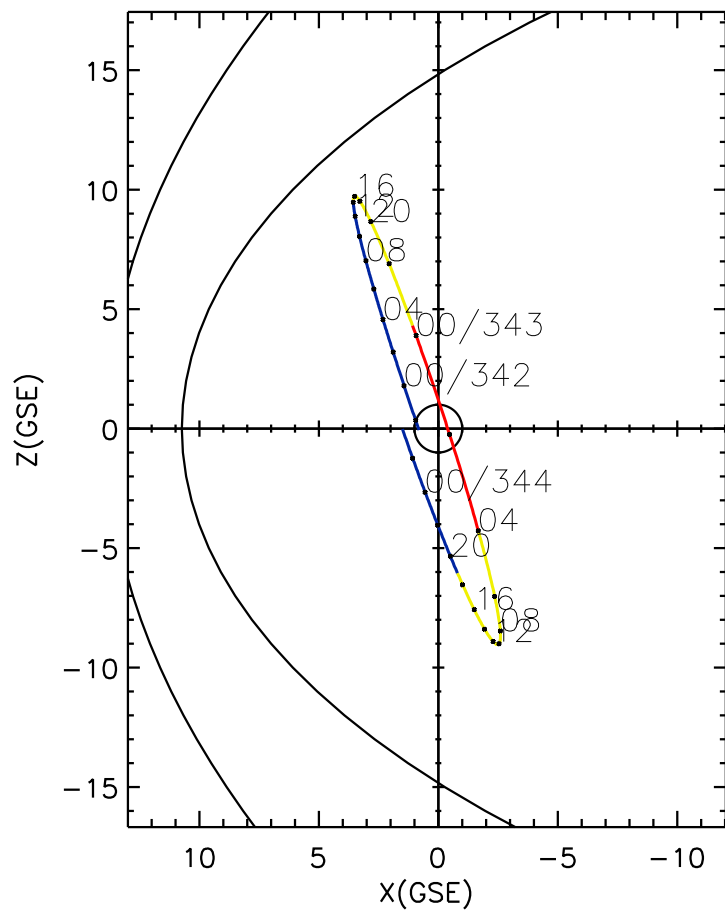
CLUSTER 2 orbit 2018 341 (12/07) 21:26 UT to 2018 344 (12/10) 03:41 UT
