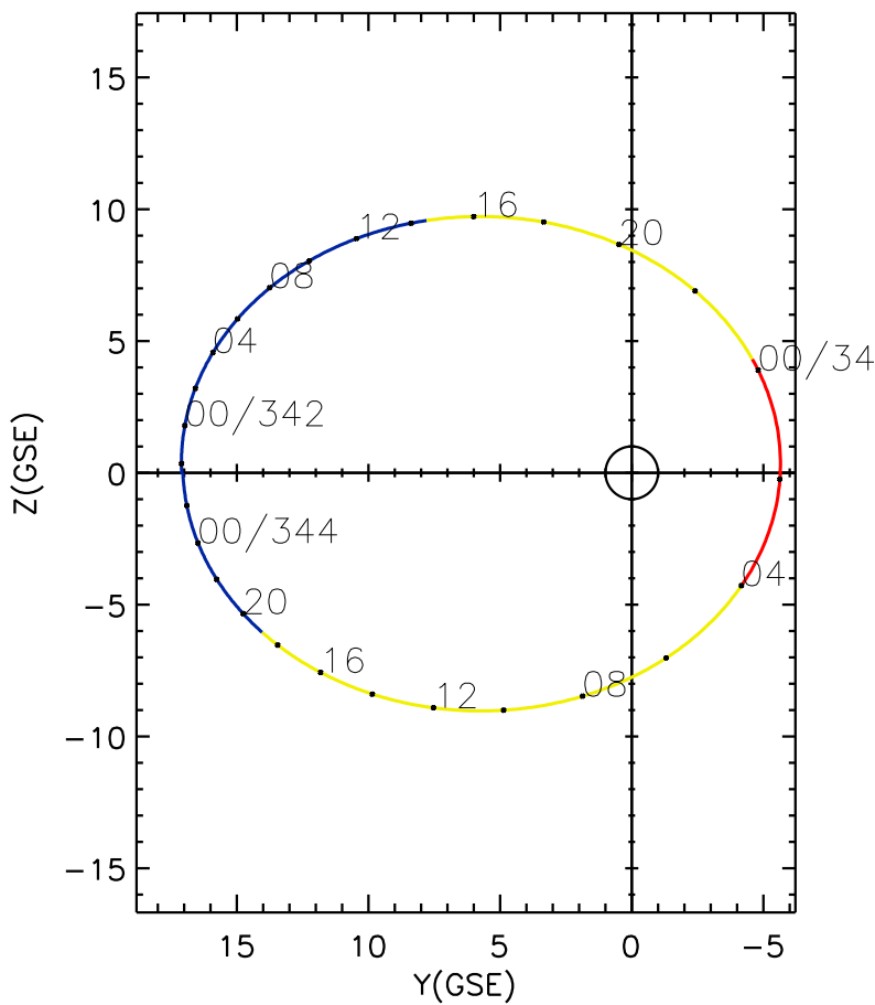
CLUSTER 2 orbit 2018 341 (12/07) 21:26 UT to 2018 344 (12/10) 03:41 UT
