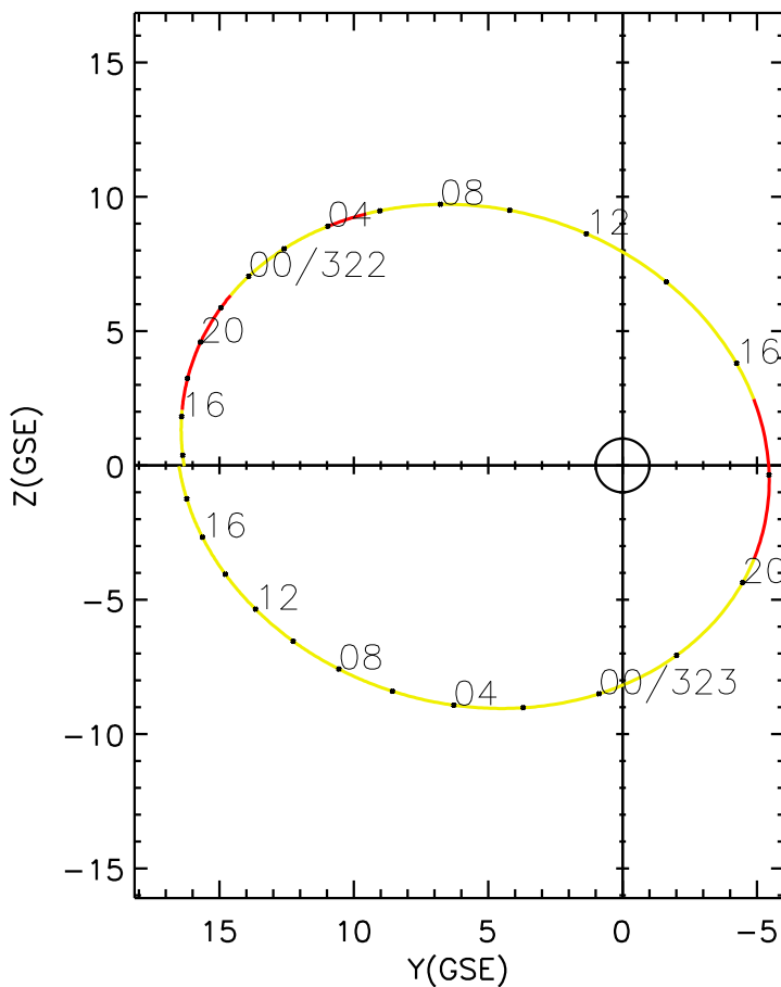
CLUSTER 2 orbit 2018 321 (11/17) 13:26 UT to 2018 323 (11/19) 19:41 UT
