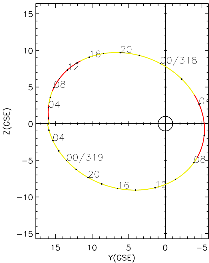
CLUSTER 2 orbit 2018 317 (11/13) 00:56 UT to 2018 319 (11/15) 07:11 UT
