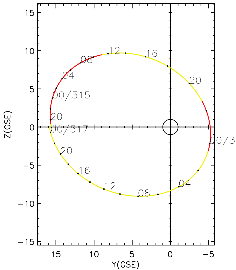
CLUSTER 2 orbit 2018 314 (11/10) 18:41 UT to 2018 317 (11/13) 00:56 UT
