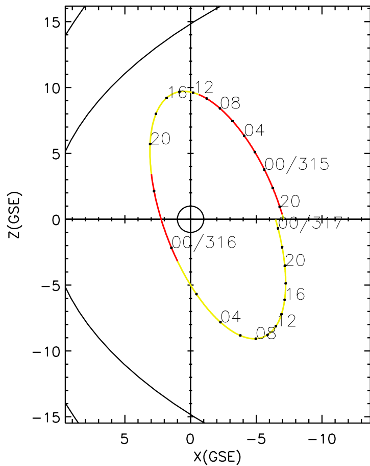
CLUSTER 2 orbit 2018 314 (11/10) 18:41 UT to 2018 317 (11/13) 00:56 UT
