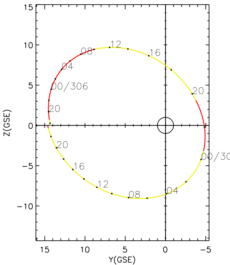
CLUSTER 2 orbit 2018 305 (11/01) 17:36 UT to 2018 307 (11/03) 23:51 UT
