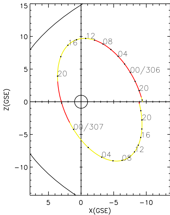
CLUSTER 2 orbit 2018 305 (11/01) 17:36 UT to 2018 307 (11/03) 23:51 UT
