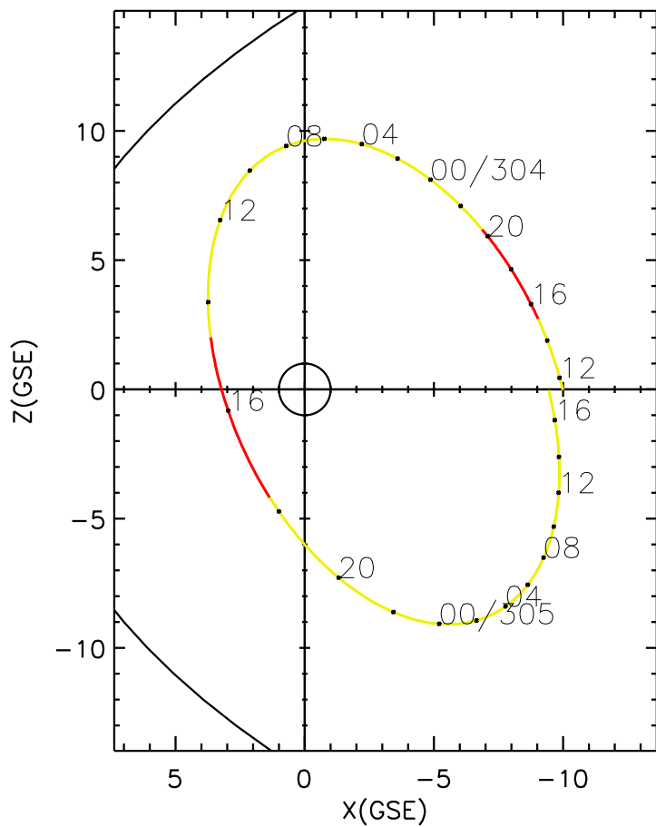
CLUSTER 2 orbit 2018 303 (10/30) 11:21 UT to 2018 305 (11/01) 17:36 UT
