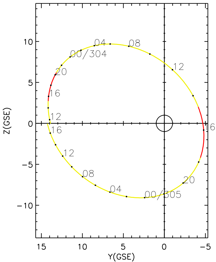
CLUSTER 2 orbit 2018 303 (10/30) 11:21 UT to 2018 305 (11/01) 17:36 UT
