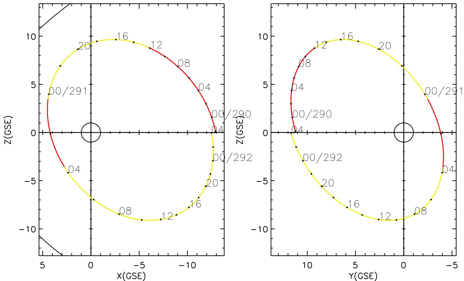
CLUSTER 2 orbit 2018 289 (10/16) 21:46 UT to 2018 292 (10/19) 04:01 UT
