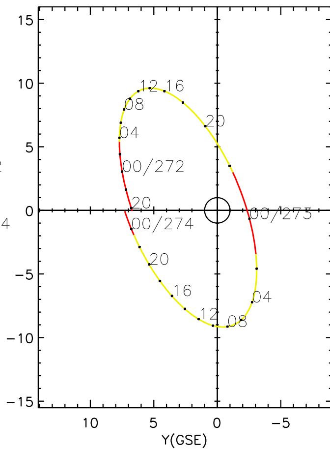
CLUSTER 2 orbit 2018 271 (09/28) 19:41 UT to 2018 274 (10/01) 01:56 UT
