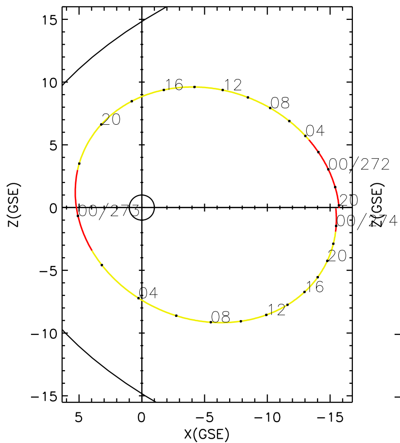
CLUSTER 2 orbit 2018 271 (09/28) 19:41 UT to 2018 274 (10/01) 01:56 UT
