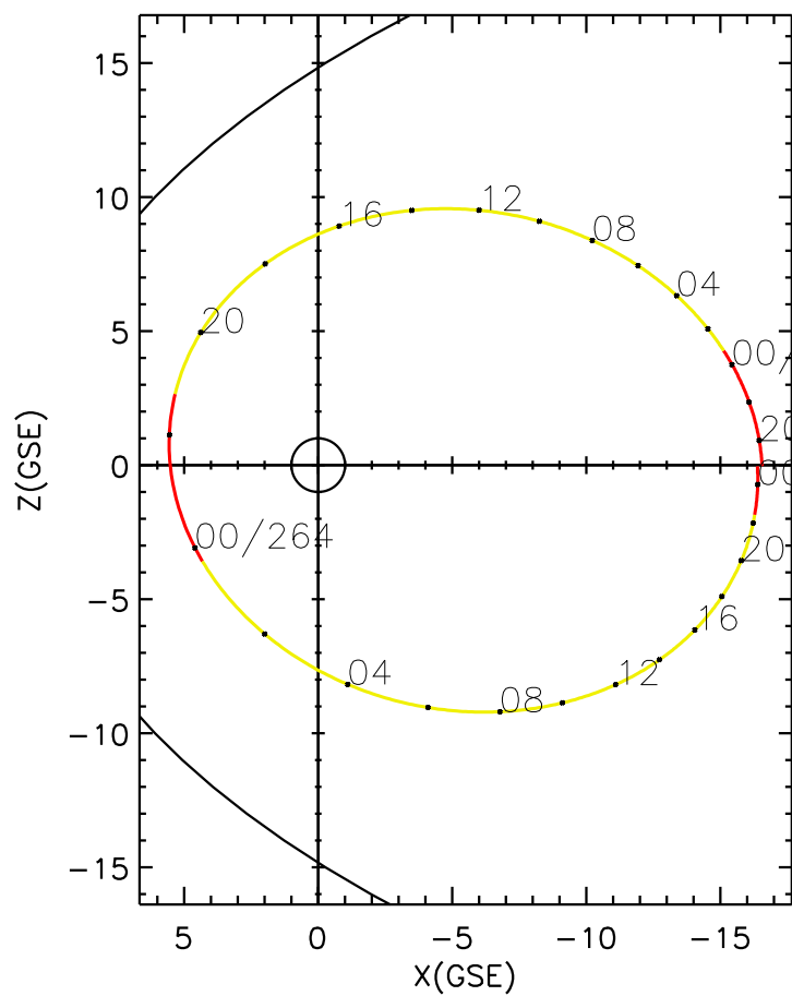
CLUSTER 2 orbit 2018 262 (09/19) 18:41 UT to 2018 265 (09/22) 00:56 UT
