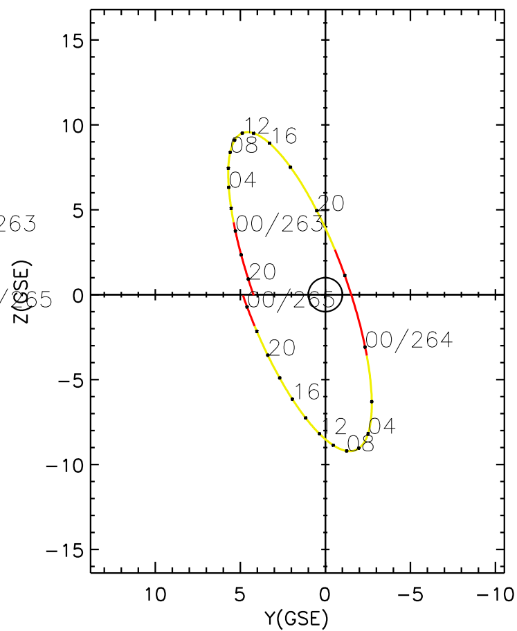
CLUSTER 2 orbit 2018 262 (09/19) 18:41 UT to 2018 265 (09/22) 00:56 UT
