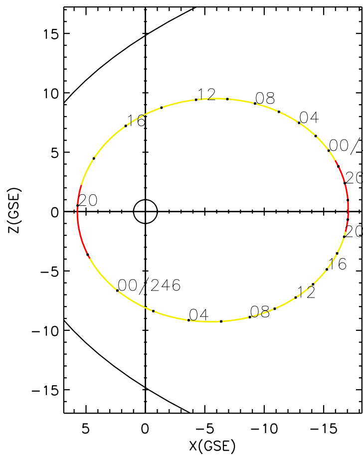
CLUSTER 2 orbit 2018 244 (09/01) 16:36 UT to 2018 246 (09/03) 22:51 UT
