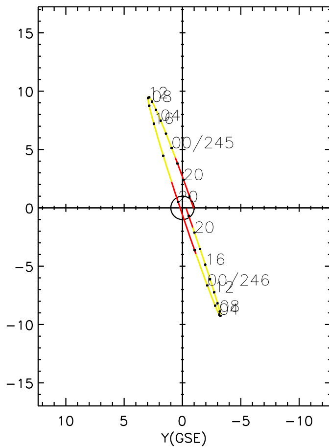
CLUSTER 2 orbit 2018 244 (09/01) 16:36 UT to 2018 246 (09/03) 22:51 UT
