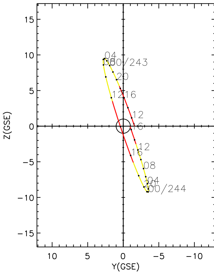
CLUSTER 2 orbit 2018 242 (08/30) 10:21 UT to 2018 244 (09/01) 16:36 UT
