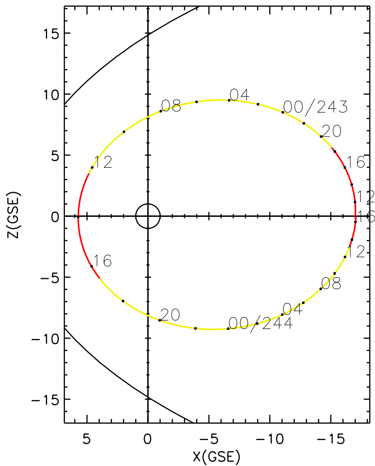
CLUSTER 2 orbit 2018 242 (08/30) 10:21 UT to 2018 244 (09/01) 16:36 UT
