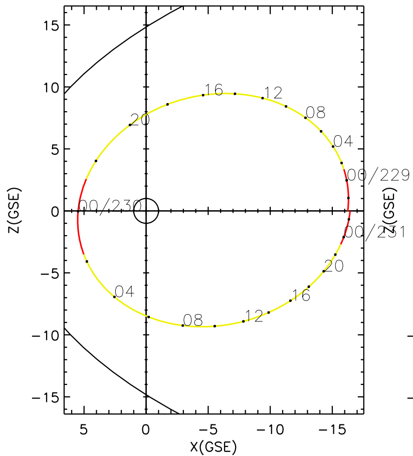
CLUSTER 2 orbit 2018 228 (08/16) 20:31 UT to 2018 231 (08/19) 02:56 UT
