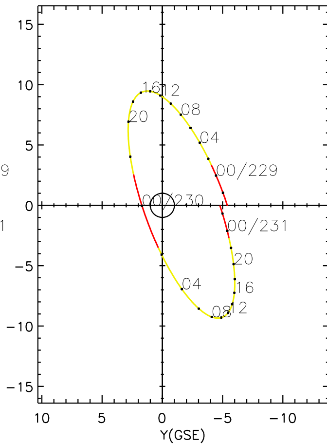
CLUSTER 2 orbit 2018 228 (08/16) 20:31 UT to 2018 231 (08/19) 02:56 UT
