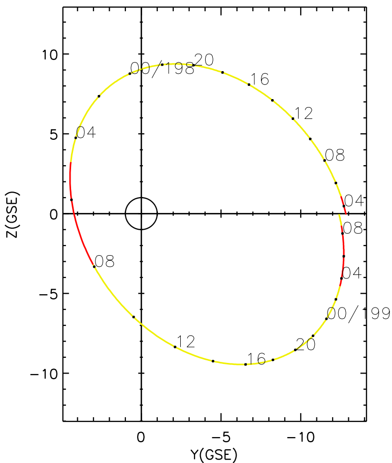
CLUSTER 2 orbit 2018 197 (07/16) 03:16 UT to 2018 199 (07/18) 09:41 UT
