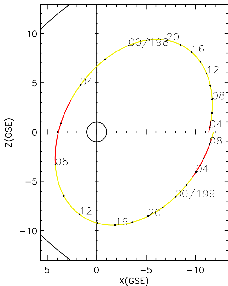
CLUSTER 2 orbit 2018 197 (07/16) 03:16 UT to 2018 199 (07/18) 09:41 UT
