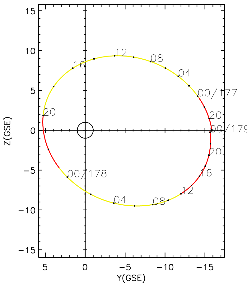
CLUSTER 2 orbit 2018 176 (06/25) 17:56 UT to 2018 179 (06/28) 00:16 UT
