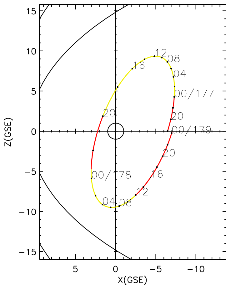
CLUSTER 2 orbit 2018 176 (06/25) 17:56 UT to 2018 179 (06/28) 00:16 UT
