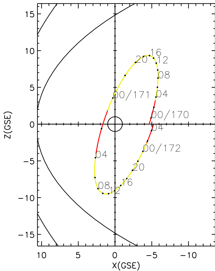
CLUSTER 2 orbit 2018 169 (06/18) 22:46 UT to 2018 172 (06/21) 05:11 UT
