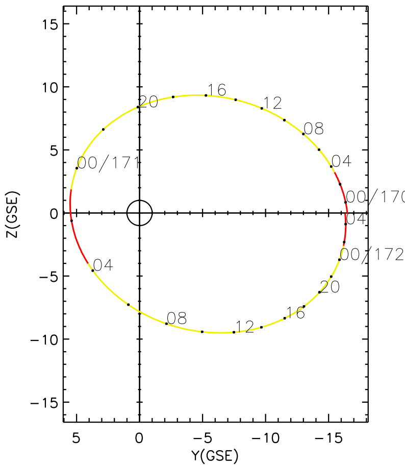
CLUSTER 2 orbit 2018 169 (06/18) 22:46 UT to 2018 172 (06/21) 05:11 UT
