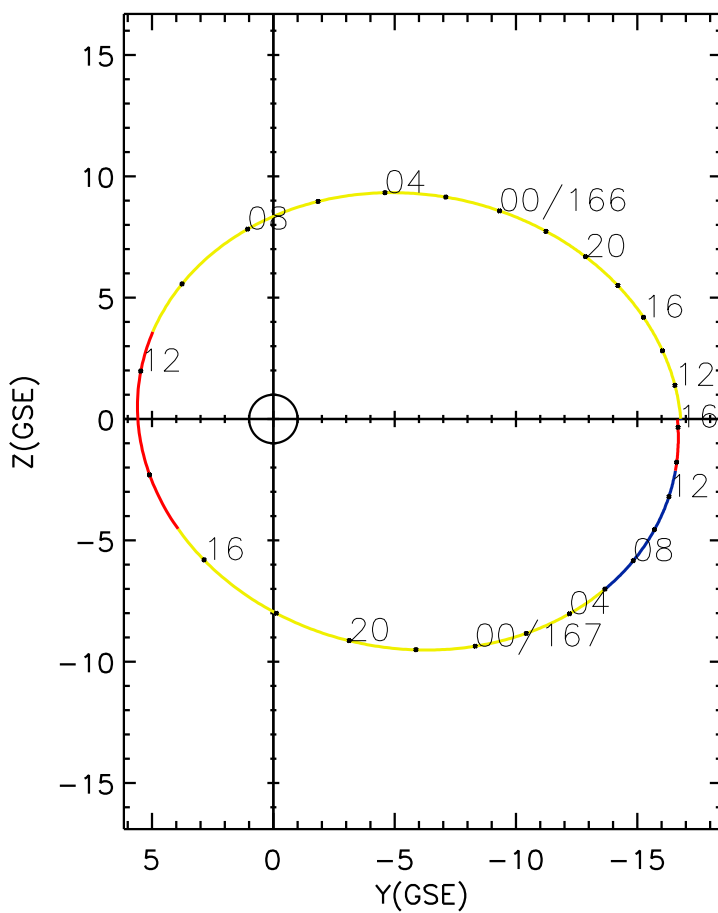
CLUSTER 2 orbit 2018 165 (06/14) 10:01 UT to 2018 167 (06/16) 16:26 UT
