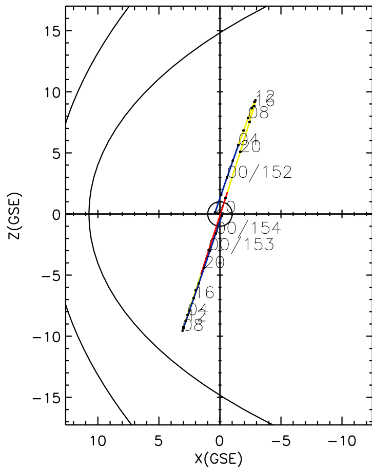
CLUSTER 2 orbit 2018 151 (05/31) 19:46 UT to 2018 154 (06/03) 02:11 UT
