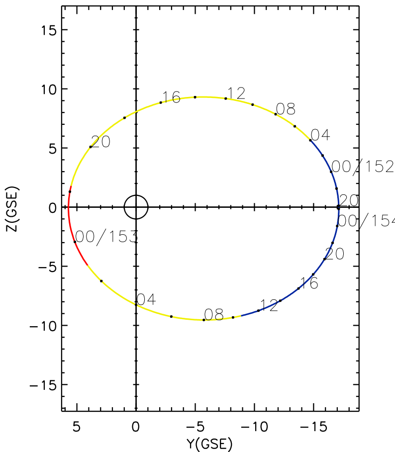
CLUSTER 2 orbit 2018 151 (05/31) 19:46 UT to 2018 154 (06/03) 02:11 UT
