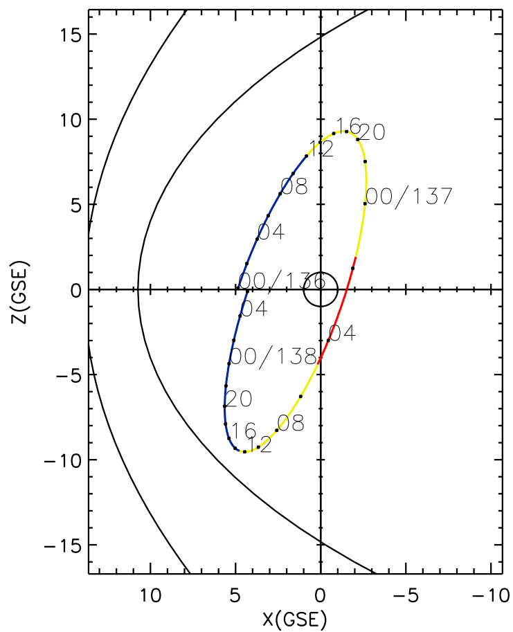
CLUSTER 2 orbit 2018 135 (05/15) 23:51 UT to 2018 138 (05/18) 06:06 UT
