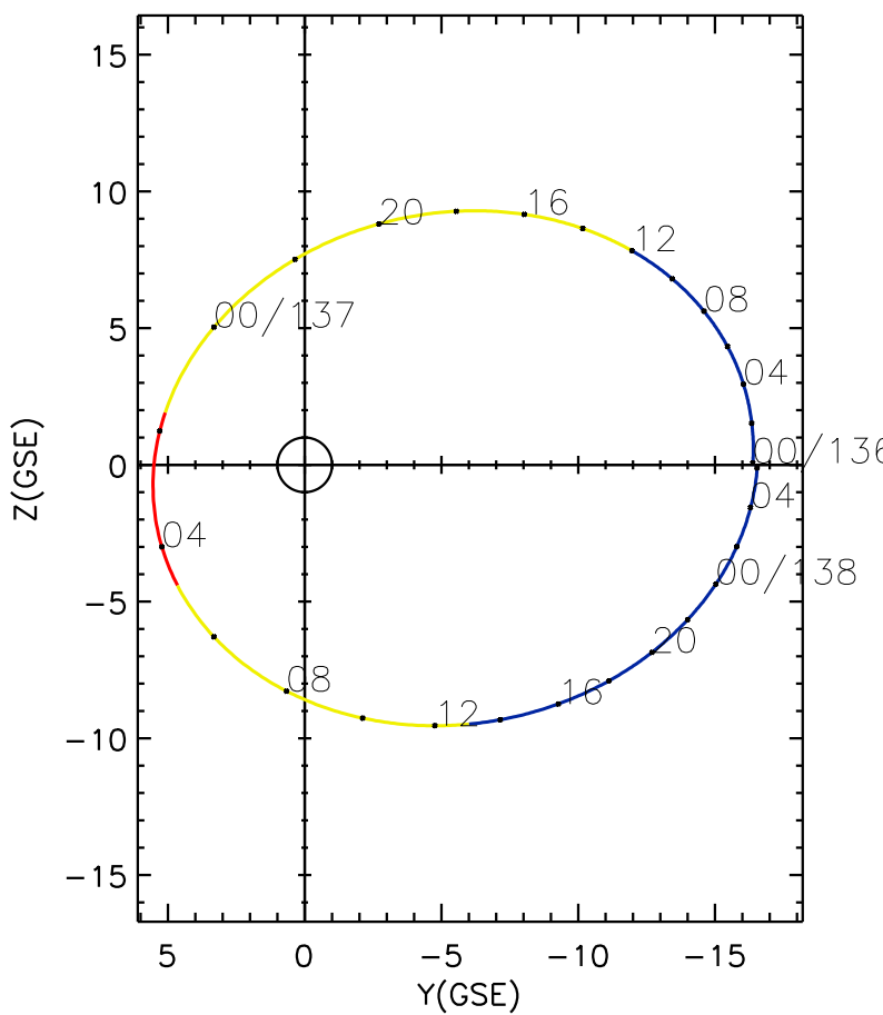
CLUSTER 2 orbit 2018 135 (05/15) 23:51 UT to 2018 138 (05/18) 06:06 UT
