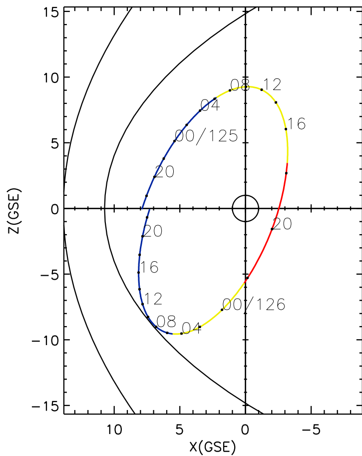
CLUSTER 2 orbit 2018 124 (05/04) 16:36 UT to 2018 126 (05/06) 22:51 UT
