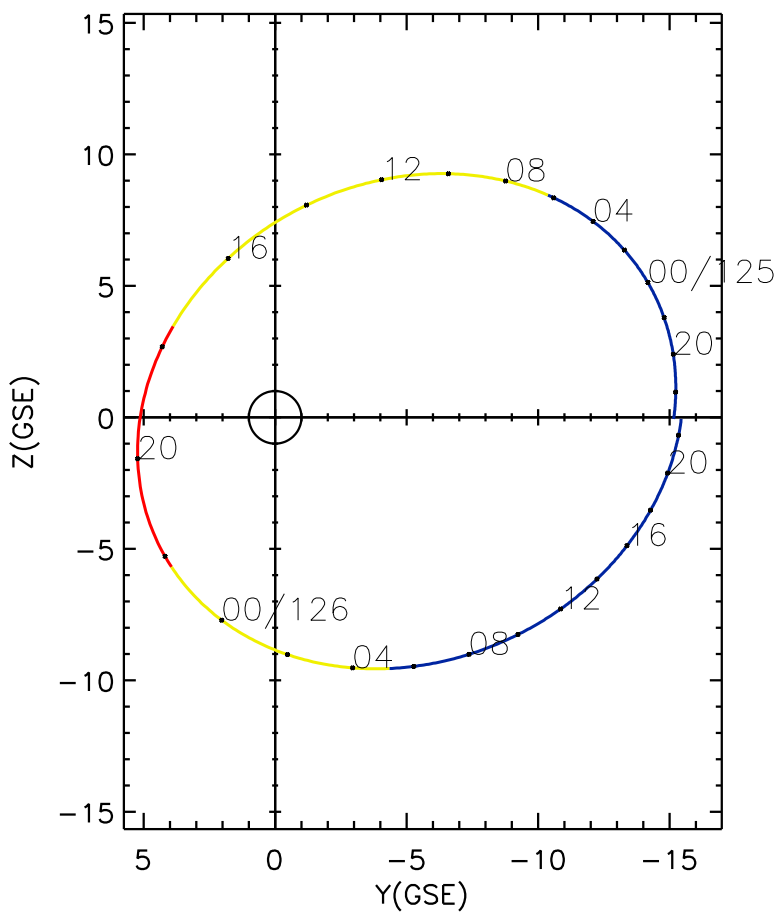
CLUSTER 2 orbit 2018 124 (05/04) 16:36 UT to 2018 126 (05/06) 22:51 UT
