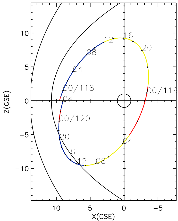
CLUSTER 2 orbit 2018 117 (04/27) 21:51 UT to 2018 120 (04/30) 04:06 UT
