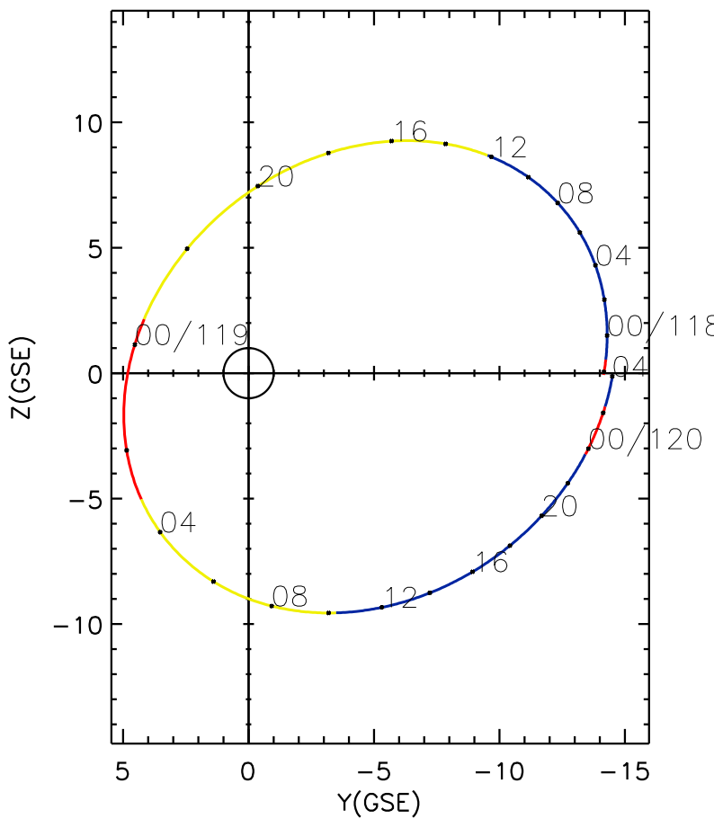
CLUSTER 2 orbit 2018 117 (04/27) 21:51 UT to 2018 120 (04/30) 04:06 UT
