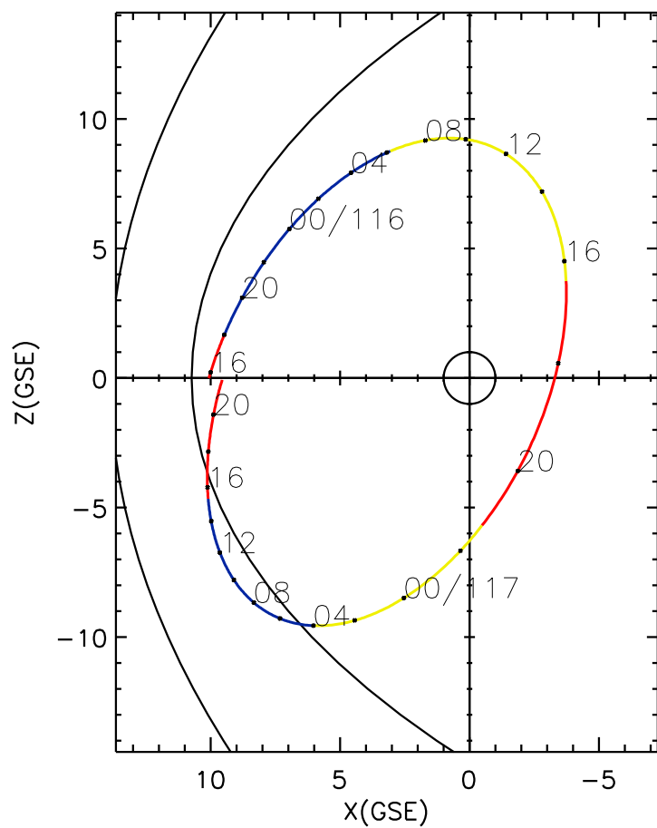
CLUSTER 2 orbit 2018 115 (04/25) 15:41 UT to 2018 117 (04/27) 21:51 UT
