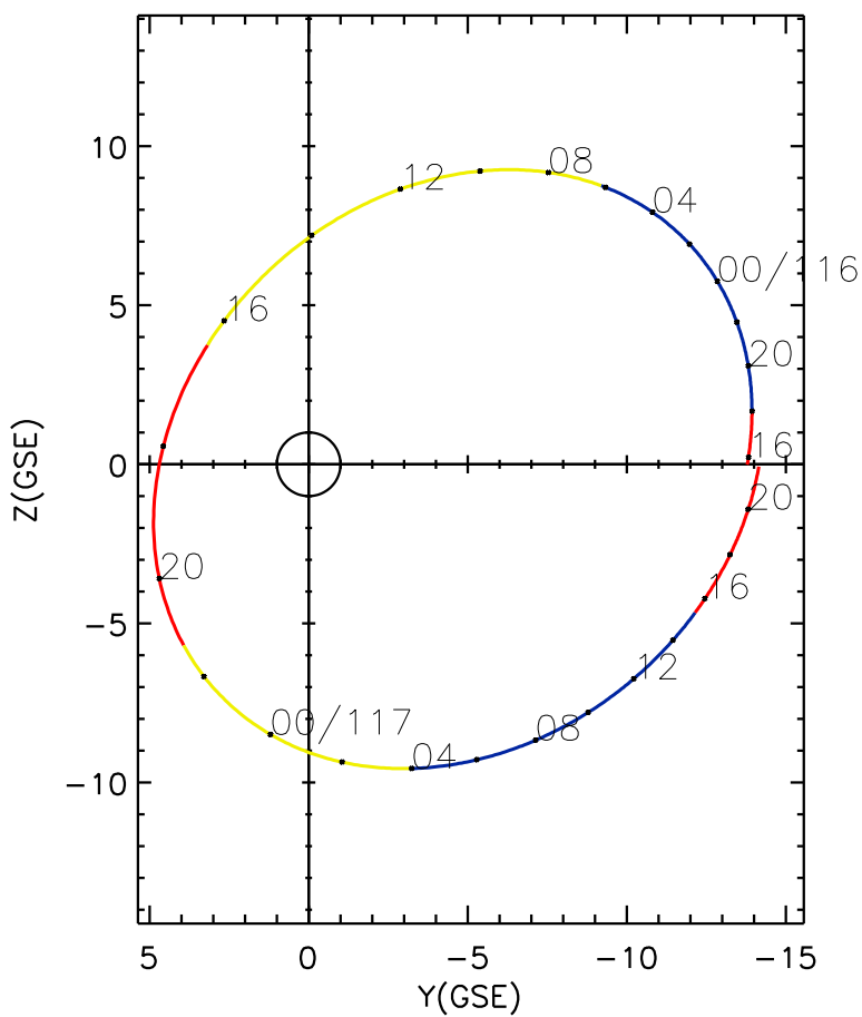
CLUSTER 2 orbit 2018 115 (04/25) 15:41 UT to 2018 117 (04/27) 21:51 UT
