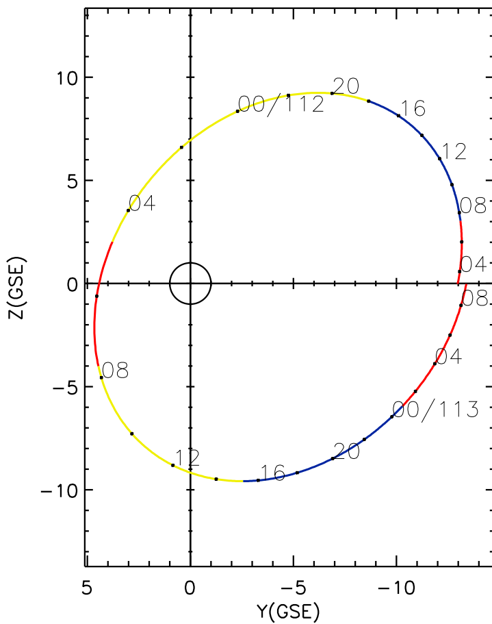
CLUSTER 2 orbit 2018 111 (04/21) 03:11 UT to 2018 113 (04/23) 09:26 UT
