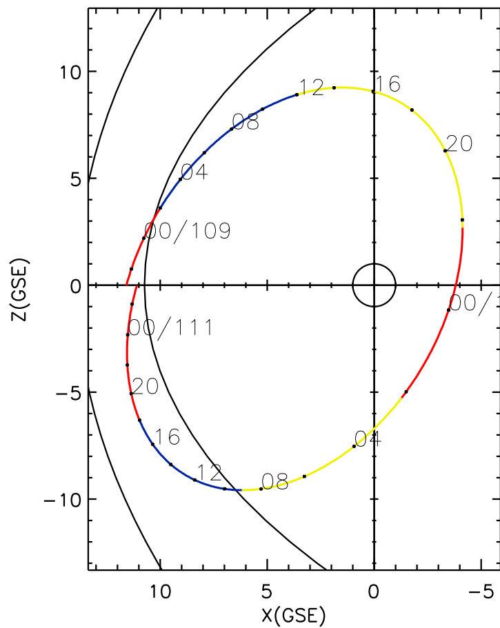
CLUSTER 2 orbit 2018 108 (04/18) 20:56 UT to 2018 111 (04/21) 03:11 UT
