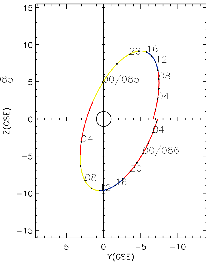
CLUSTER 2 orbit 2018 084 (03/25) 00:16 UT to 2018 086 (03/27) 06:31 UT
