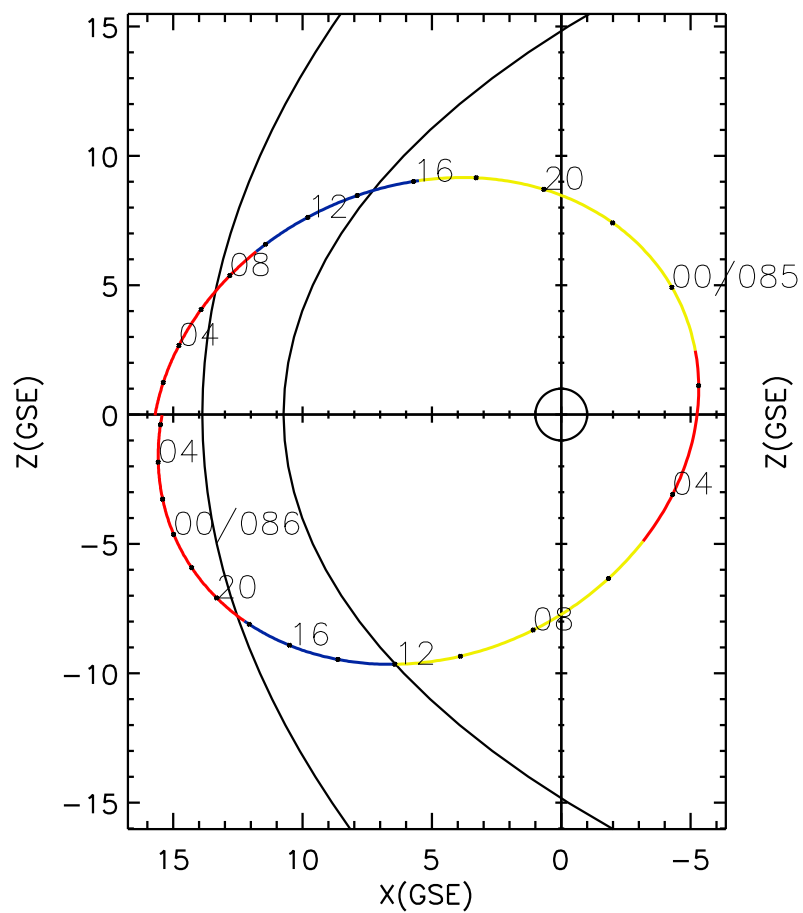
CLUSTER 2 orbit 2018 084 (03/25) 00:16 UT to 2018 086 (03/27) 06:31 UT
