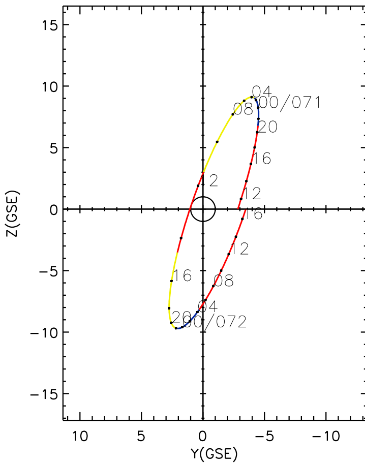
CLUSTER 2 orbit 2018 070 (03/11) 10:51 UT to 2018 072 (03/13) 17:06 UT
