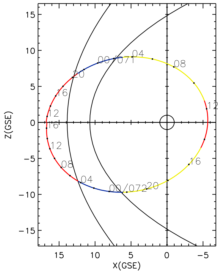
CLUSTER 2 orbit 2018 070 (03/11) 10:51 UT to 2018 072 (03/13) 17:06 UT
