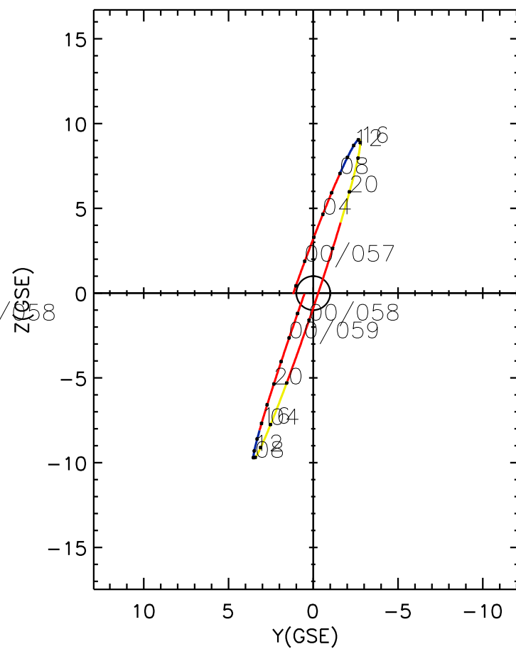
CLUSTER 2 orbit 2018 056 (02/25) 21:21 UT to 2018 059 (02/28) 03:36 UT
