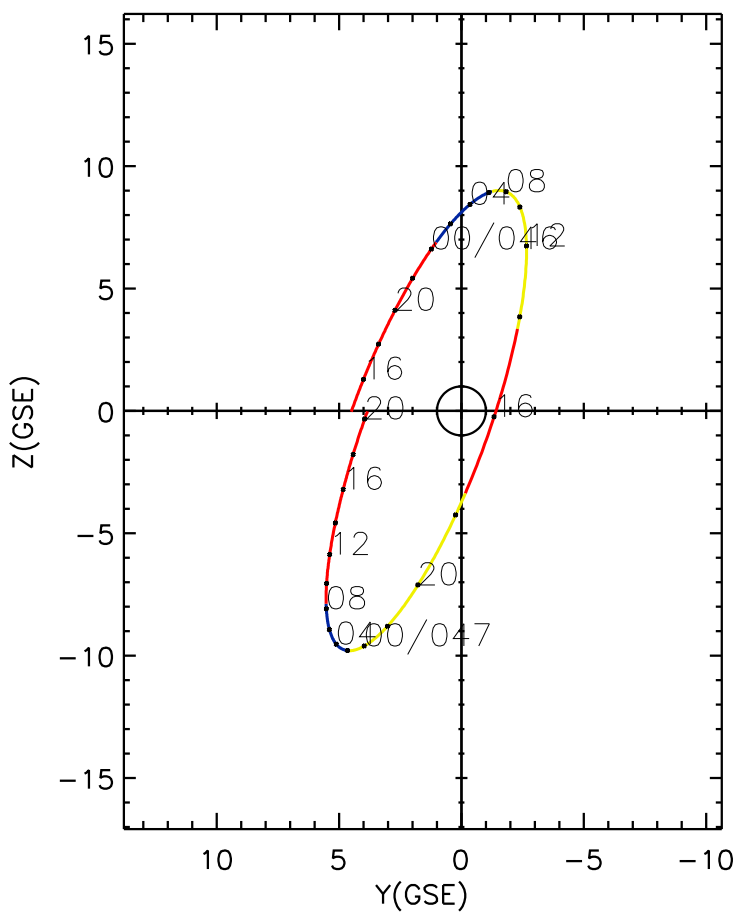
CLUSTER 2 orbit 2018 045 (02/14) 14:11 UT to 2018 047 (02/16) 20:26 UT
