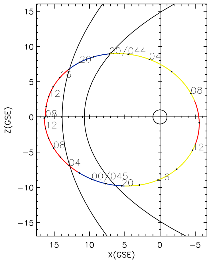
CLUSTER 2 orbit 2018 043 (02/12) 07:56 UT to 2018 045 (02/14) 14:11 UT
