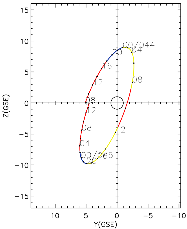
CLUSTER 2 orbit 2018 043 (02/12) 07:56 UT to 2018 045 (02/14) 14:11 UT
