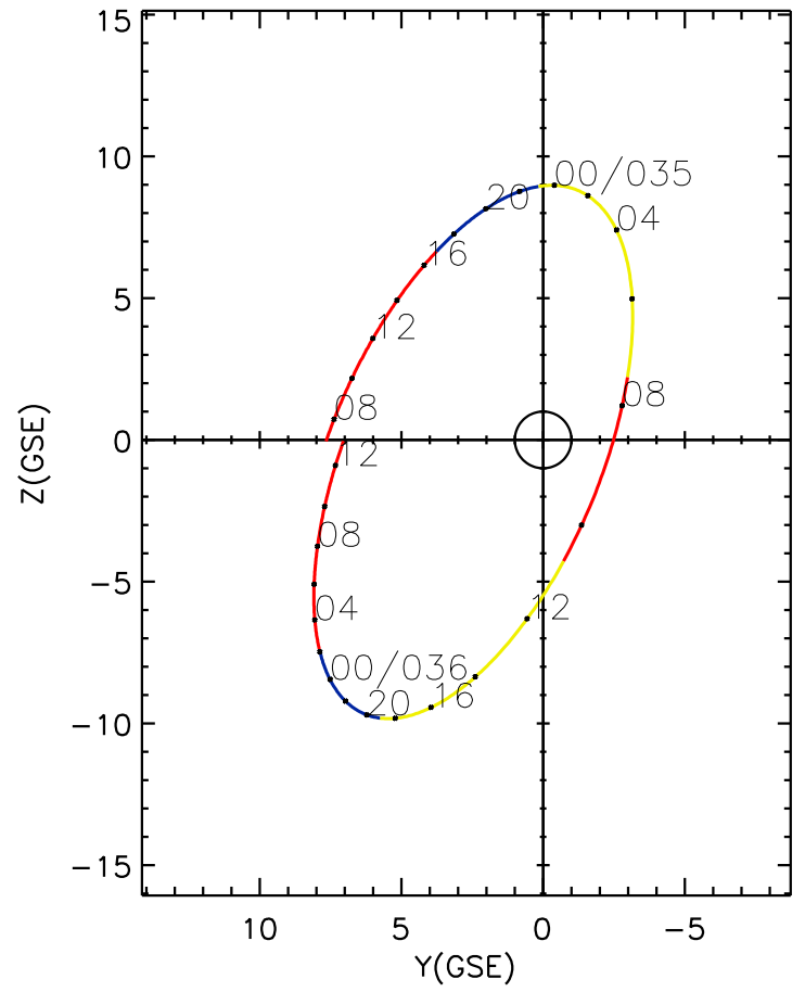
CLUSTER 2 orbit 2018 034 (02/03) 06:56 UT to 2018 036 (02/05) 13:11 UT
