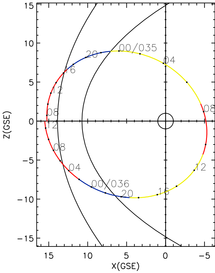
CLUSTER 2 orbit 2018 034 (02/03) 06:56 UT to 2018 036 (02/05) 13:11 UT
