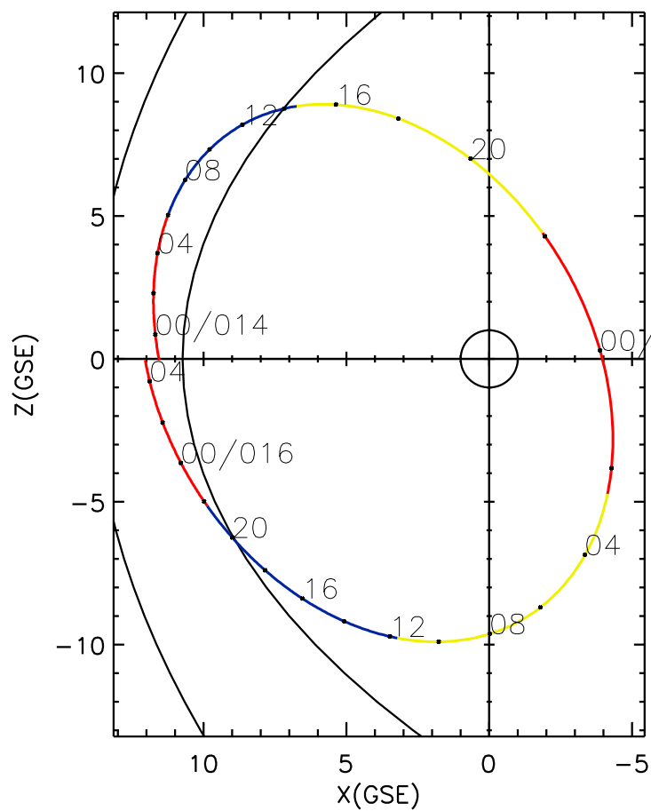
CLUSTER 2 orbit 2018 013 (01/13) 22:46 UT to 2018 016 (01/16) 05:01 UT
