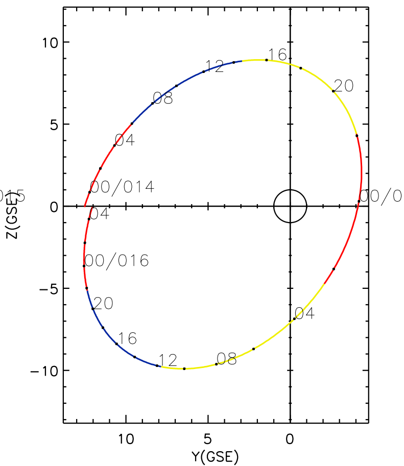
CLUSTER 2 orbit 2018 013 (01/13) 22:46 UT to 2018 016 (01/16) 05:01 UT
