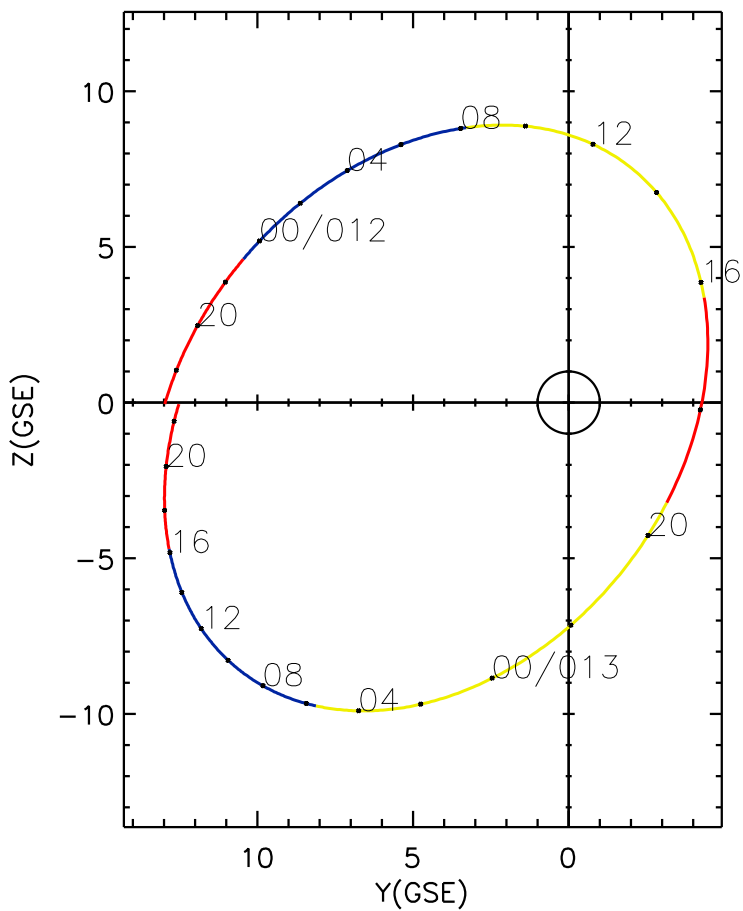
CLUSTER 2 orbit 2018 011 (01/11) 16:31 UT to 2018 013 (01/13) 22:46 UT
