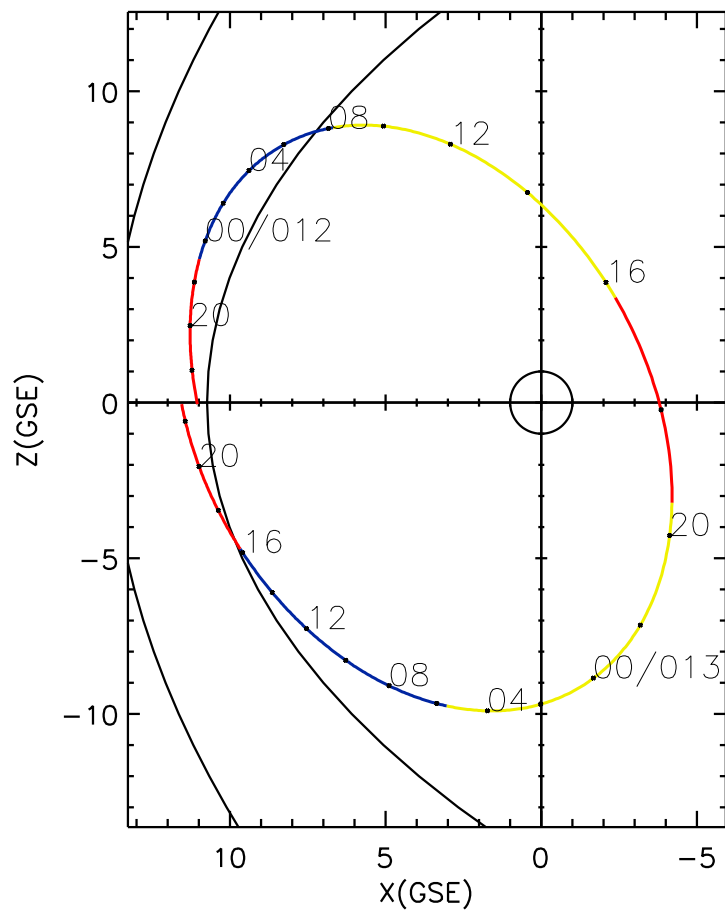
CLUSTER 2 orbit 2018 011 (01/11) 16:31 UT to 2018 013 (01/13) 22:46 UT
