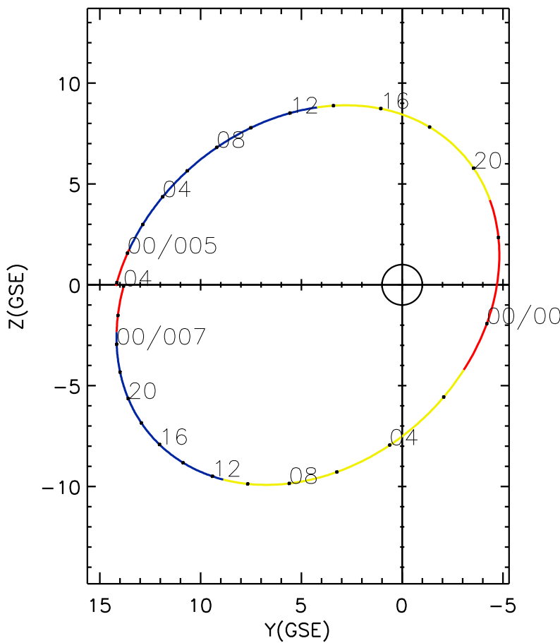
CLUSTER 2 orbit 2018 004 (01/04) 21:46 UT to 2018 007 (01/07) 04:01 UT
