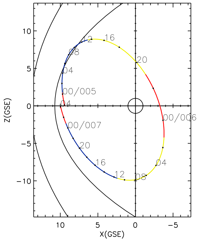
CLUSTER 2 orbit 2018 004 (01/04) 21:46 UT to 2018 007 (01/07) 04:01 UT
