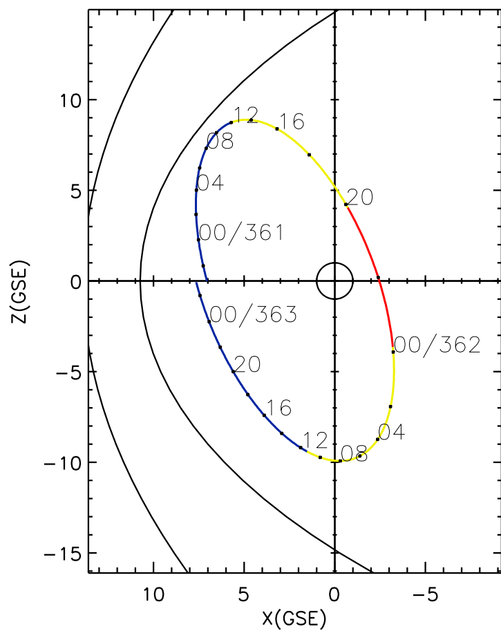
CLUSTER 2 orbit 2017 360 (12/26) 20:51 UT to 2017 363 (12/29) 03:01 UT
