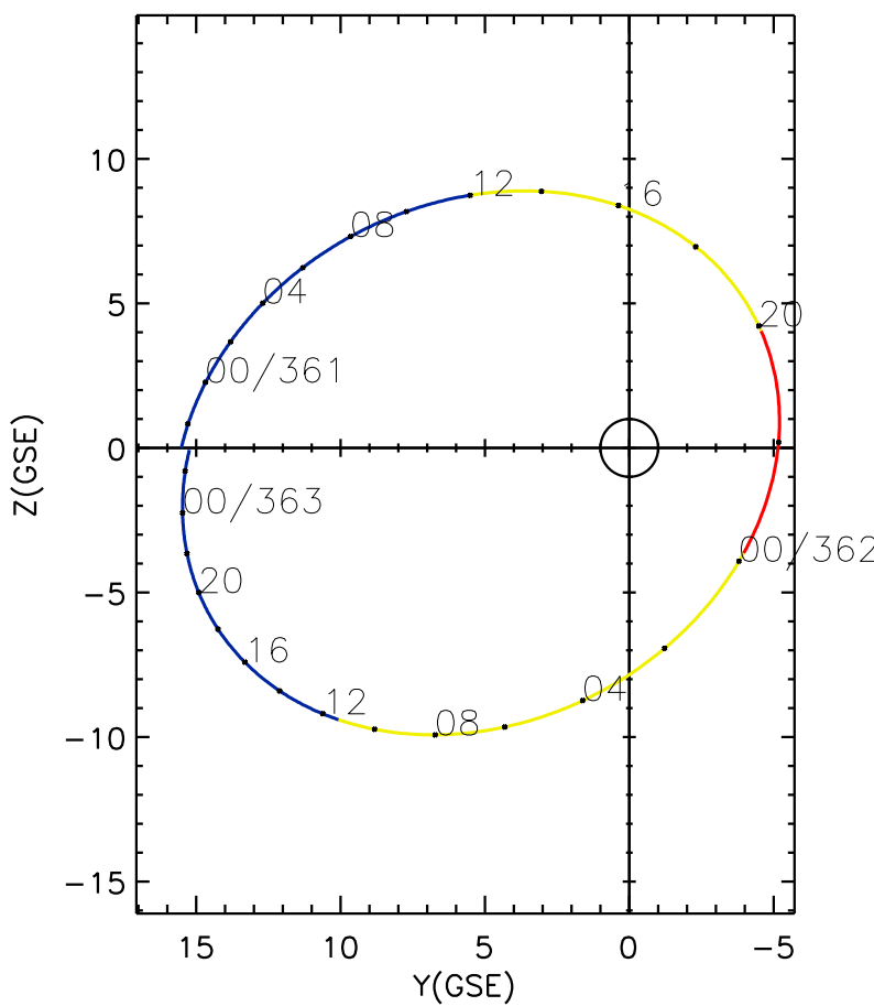
CLUSTER 2 orbit 2017 360 (12/26) 20:51 UT to 2017 363 (12/29) 03:01 UT
